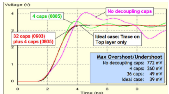
FIGURE 5. The effects of decoupling capacitors for multi-layer bus routing.
